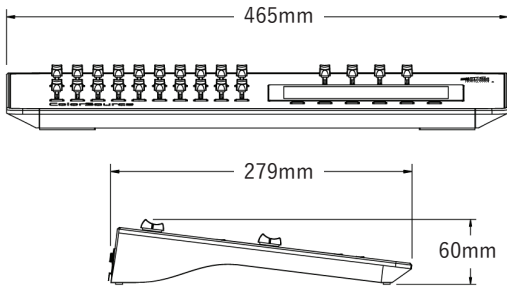
ColorSource 20
