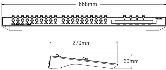
ColorSource 40
